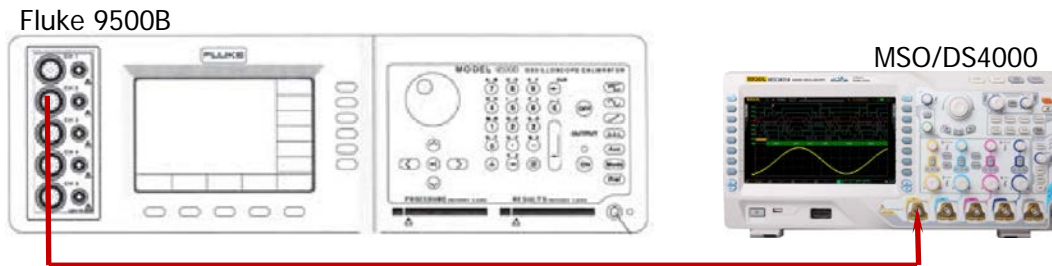
Figure 2-6 Zero Point Offset Test Connection Diagram
